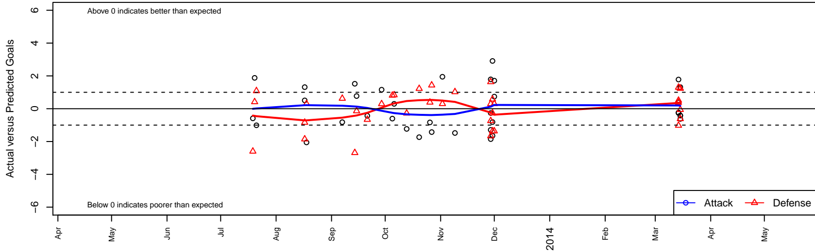
IE Surf B97 Dots are actual minus expected GF (blue circles) and GA (red triangles). Blue line is smoothed change in attack strength. Red is smoothed change in defense strength.
